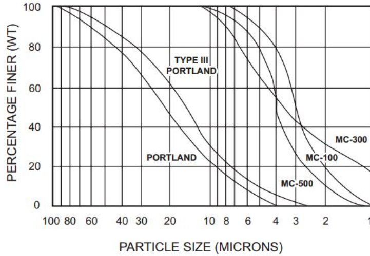
DeNeef Ultra Fine Cement Chart
