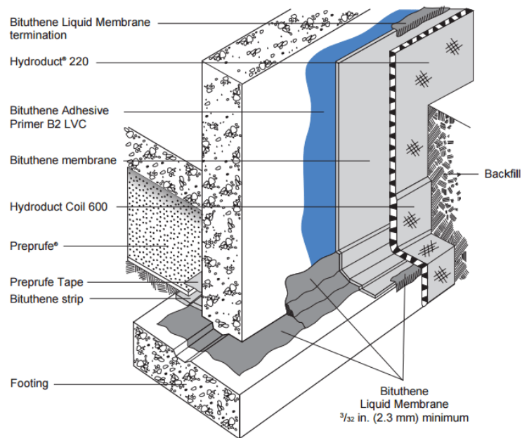
Figure of Bituthene Adhesive Primer B2 LVC Application
