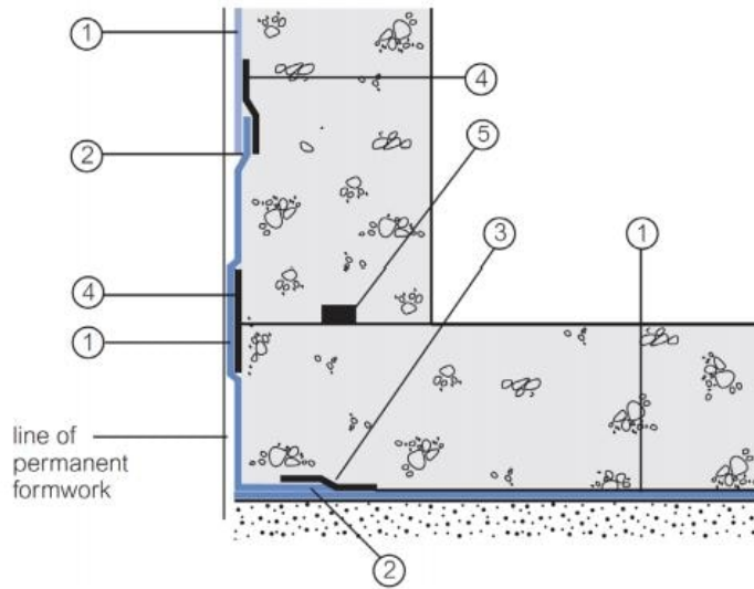
Preprufe GMA Wall Base Detail Against Permanent Shutter
