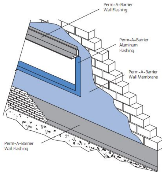
Perm-A-Barrier Aluminum Flash Application
