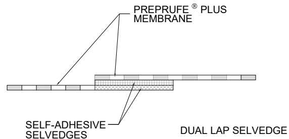
FINISHED (PLAN OR SECTION VIEW)
