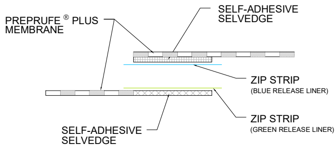
ASSEMBLY (PLAN OR SECTION VIEW)
